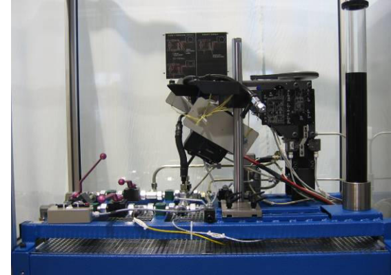
Steering gear servo pump tester
